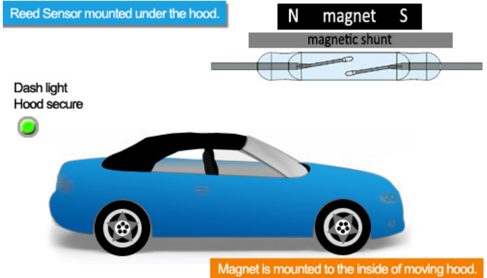
Figure 2. Reed Sensor is mounted inside engine compartment and magnet is mounted to the underside of the hood. A spring loaded ferromagnetic shunt is positioned between the sensor and magnet to shunt magnetic field.
