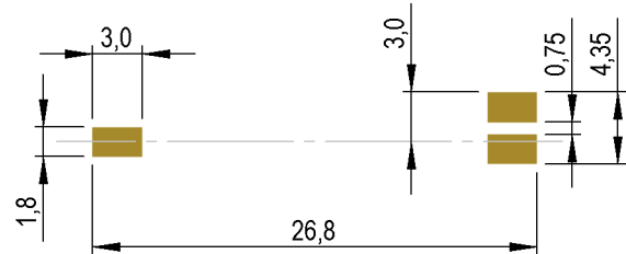
Recommended Pad Layout (mm)
